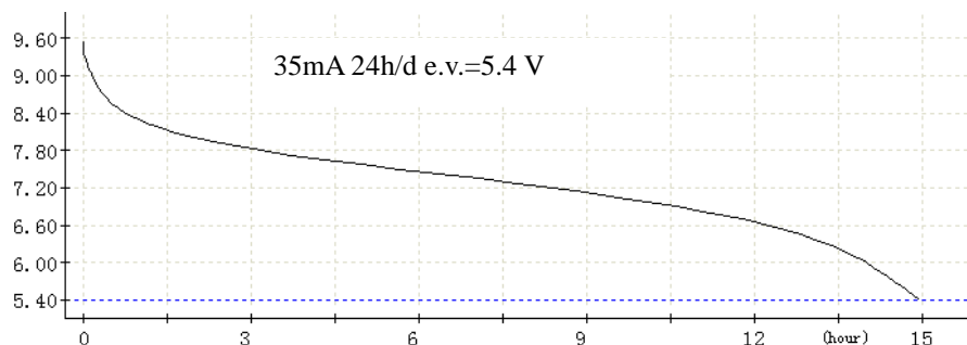
Chart 1. Discharge diagram
