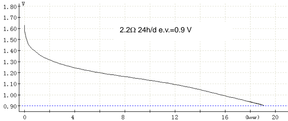
Chart 1. Discharge diagram
