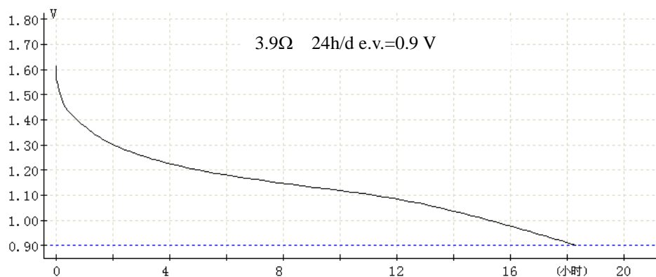
Chart 1. Discharge diagram
